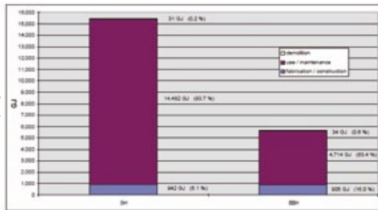
FIGURE 3-7 SH and EEH Primary Energy, total life cycle (incl. all building)
